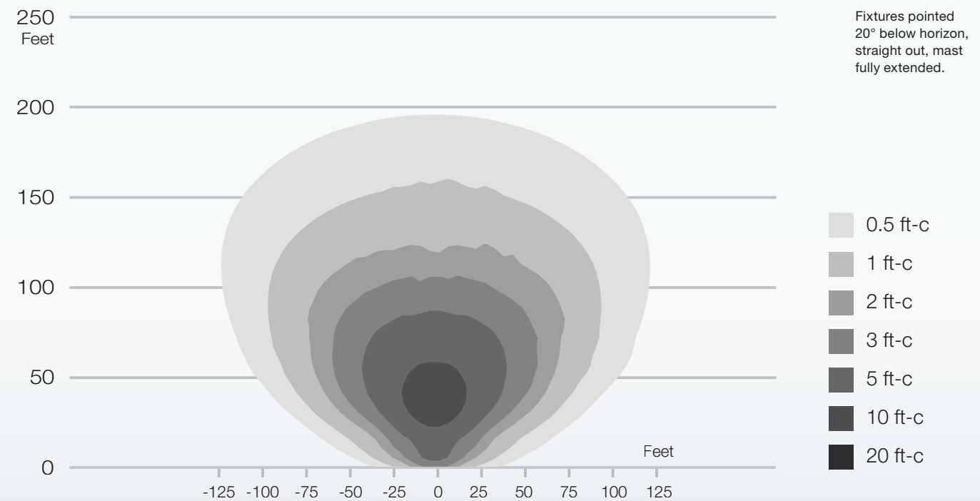
Night-Lite E-Series Manual Winch 4 – 250 W LED Light Output Area covered: 37,800 ft 2 at minimum of 0.5 ft-c
