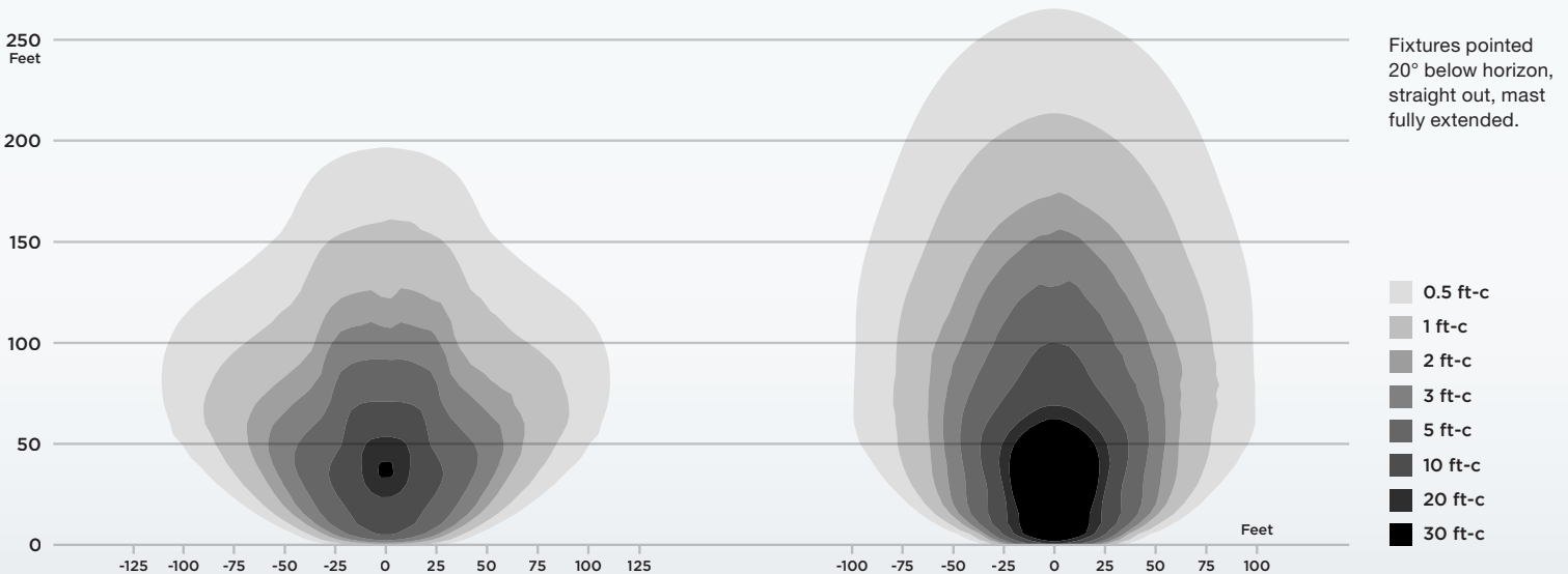
Night-Lite Pro II® LD-Series 4 – 320 W LED Light Output
